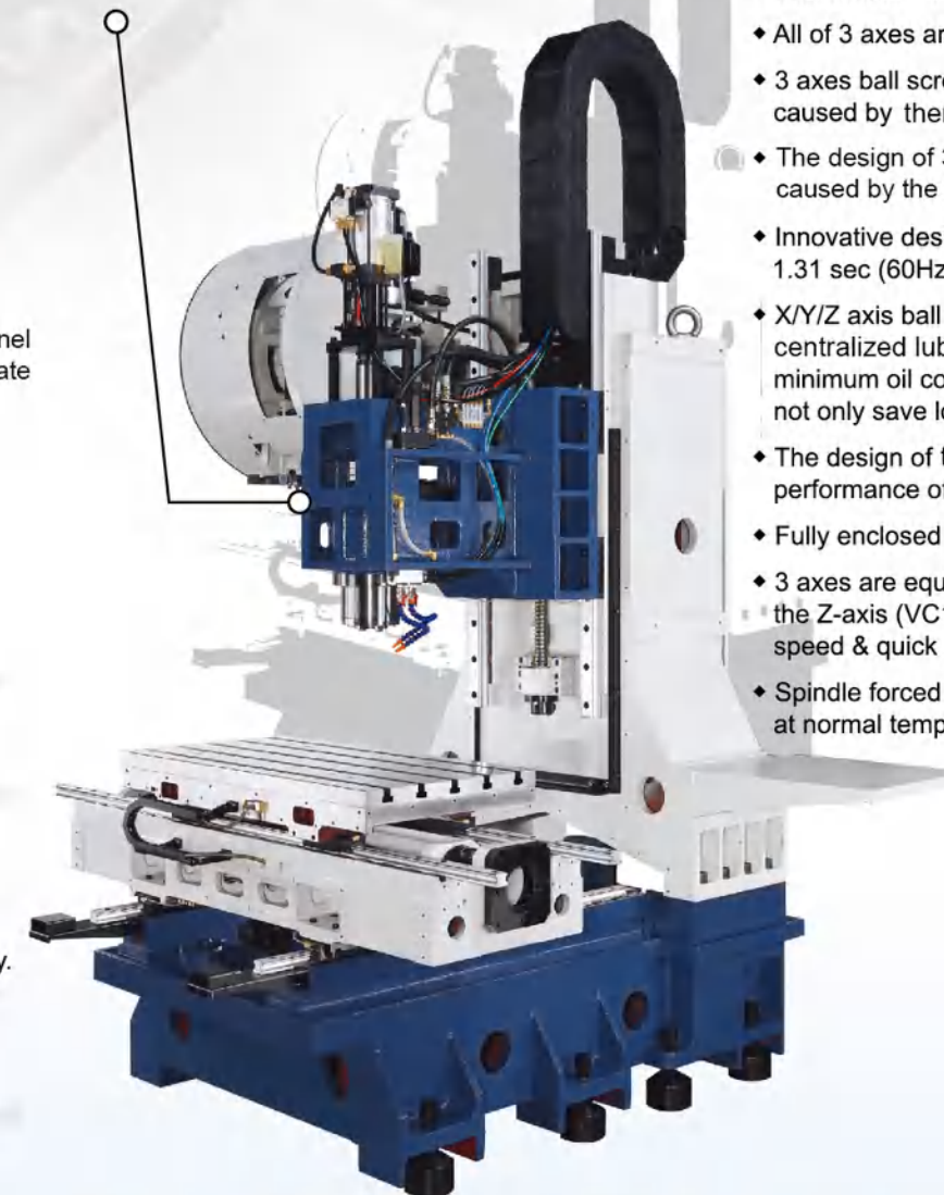
Spindle headstock is designed without counter balance to allow high speed & quick response.
