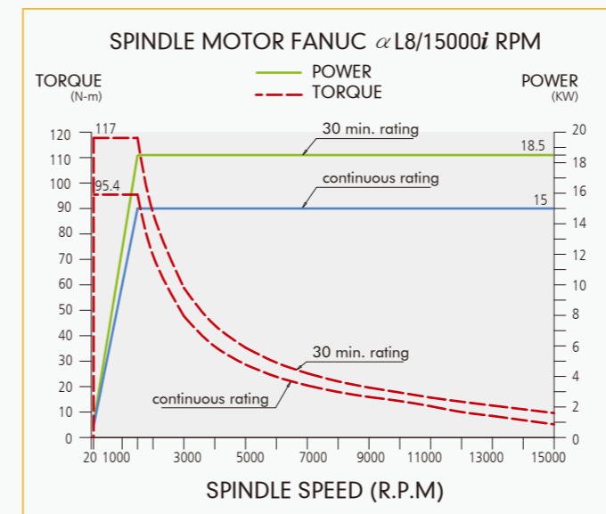
BBT40-15,000RPM DIRECT DRIVE SPINDLE (OPTIONAL)
