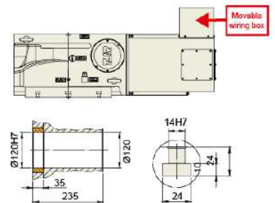
Drawing of Central Hole T-Slot Dimension
